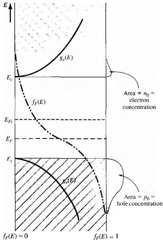
Figure 4.9 | Density of states functions, Fermi-Dirac probability function, and areas representing electron and hole concentrations for the case when E_i is below the intrinsic Fermi energy.
