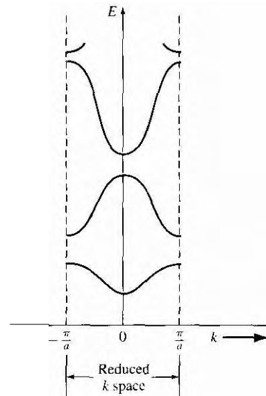
Figure 3.111 The E versus k diagram in the reduced-zone representation.
