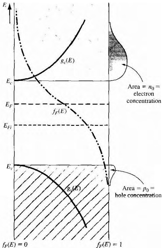
Figure 4.81 Density of states functions, Fermi–Dirac probability function, and areas representing electron and hole concentrations for the case when E_F is above the intrinsic Fermi energy.
