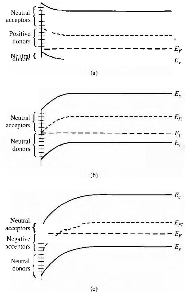
Figure 11.33 | Energy-band diagram in a p-type semiconductor showing the charge trapped in the interface states when the MOS capacitor is biased (a) in accumulation, (b) at midgap, and (c) at inversion.
