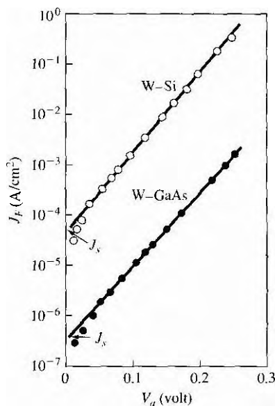
Figure 9.9 | Forward-bias current density J_F versus V_a for W-Si and W-GaAs diodes. (From Sze [14].)
