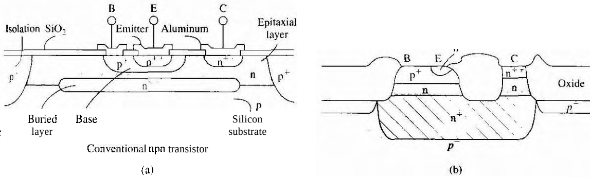
Figure 10.2 | Cross section of (a) a conventional integrated-circuit npn bipolar transistor and (b) an oxide-isolated npn bipolar transistor (Front Muller and Kamins [3].)
