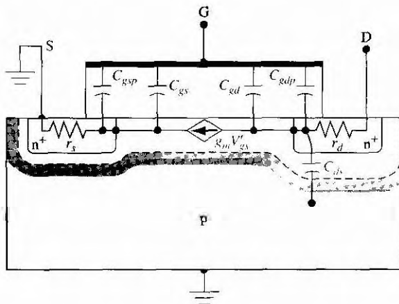
Figure 11.53 | Inherent resistances and capacitances in the n-channel MOSFET structure.
