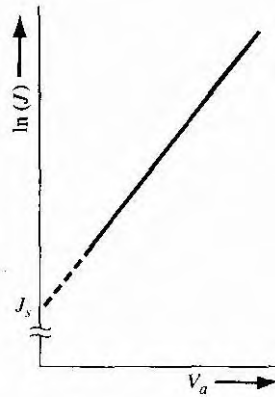
Figure 8.8 Ideal 1-V characteristic of a pn junction diode with the current plotted on a log scale.
