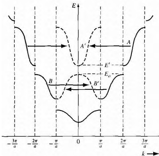
Figure 3.101 The E versus k diagram showing 2\pi displacements of several sections of allowed energy bands.
